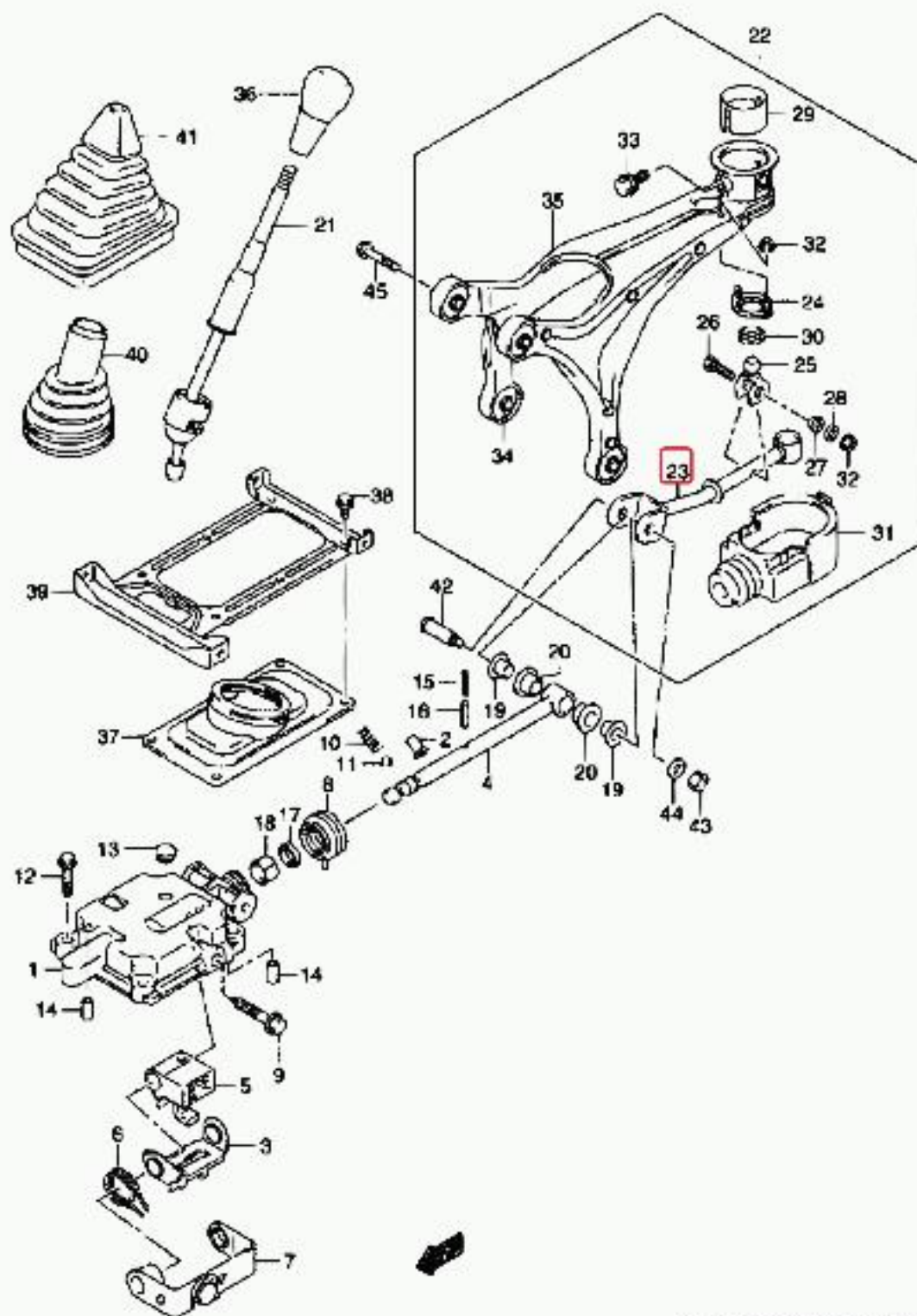
SN413-SN415D (TYPE 4)
