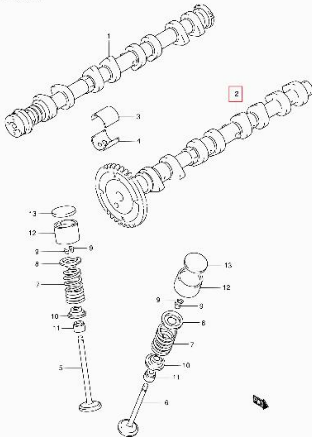
RW420 E24 036 CAM SHAFT (1)
