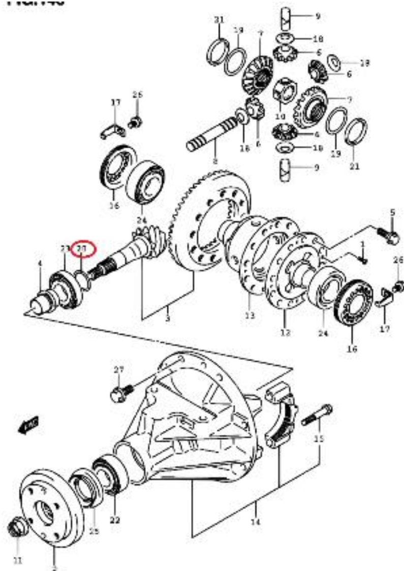
8Q420W-2 E22_146 REAR DIFF GEAR (8Q420WD:RHS:NT)
