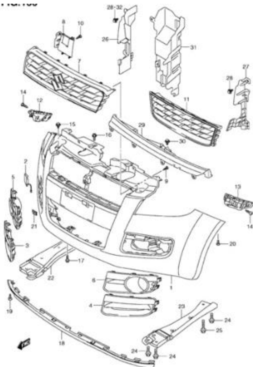
ASB310 E22_160 FRONT BUMPER
