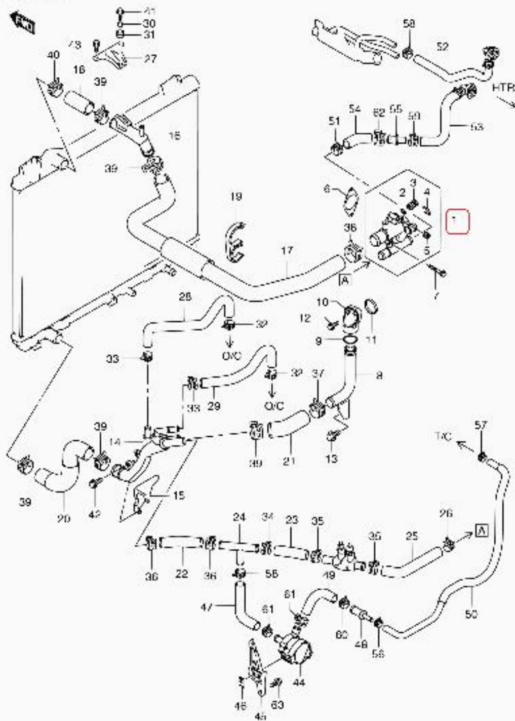
JB4116X-4 E22_060 WATER HOSE (3)
