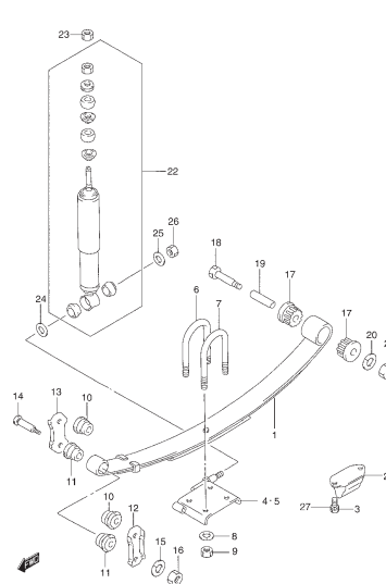
FIG. 46 SUSPENSION DELANTERA
