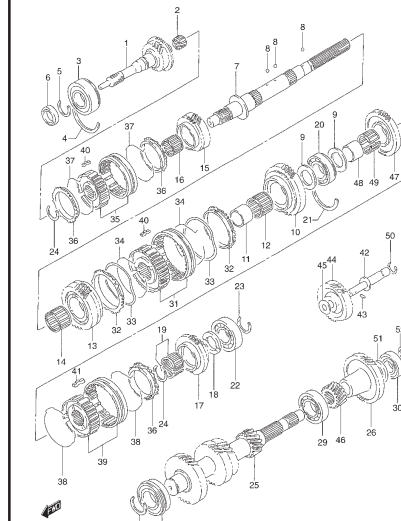
FIG. 24 TRANSMISION
