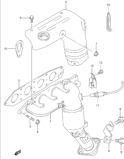
FIG. 15 COLECTOR ESCAPE
